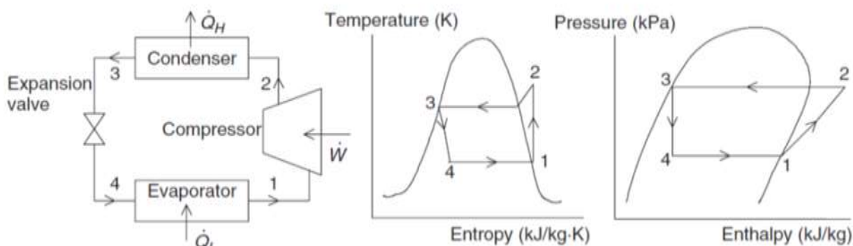
Figure 1: Block diagram T-S and p-h cycle of vapor compression system
